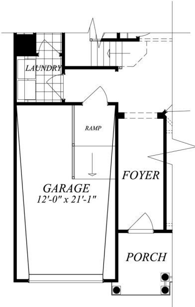
GROUND FLOOR @ HANDICAP RAMP OPTION
